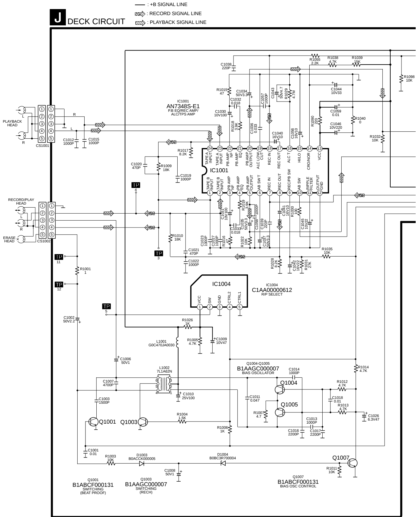
SCHEMATIC DIAGRAM - 32
