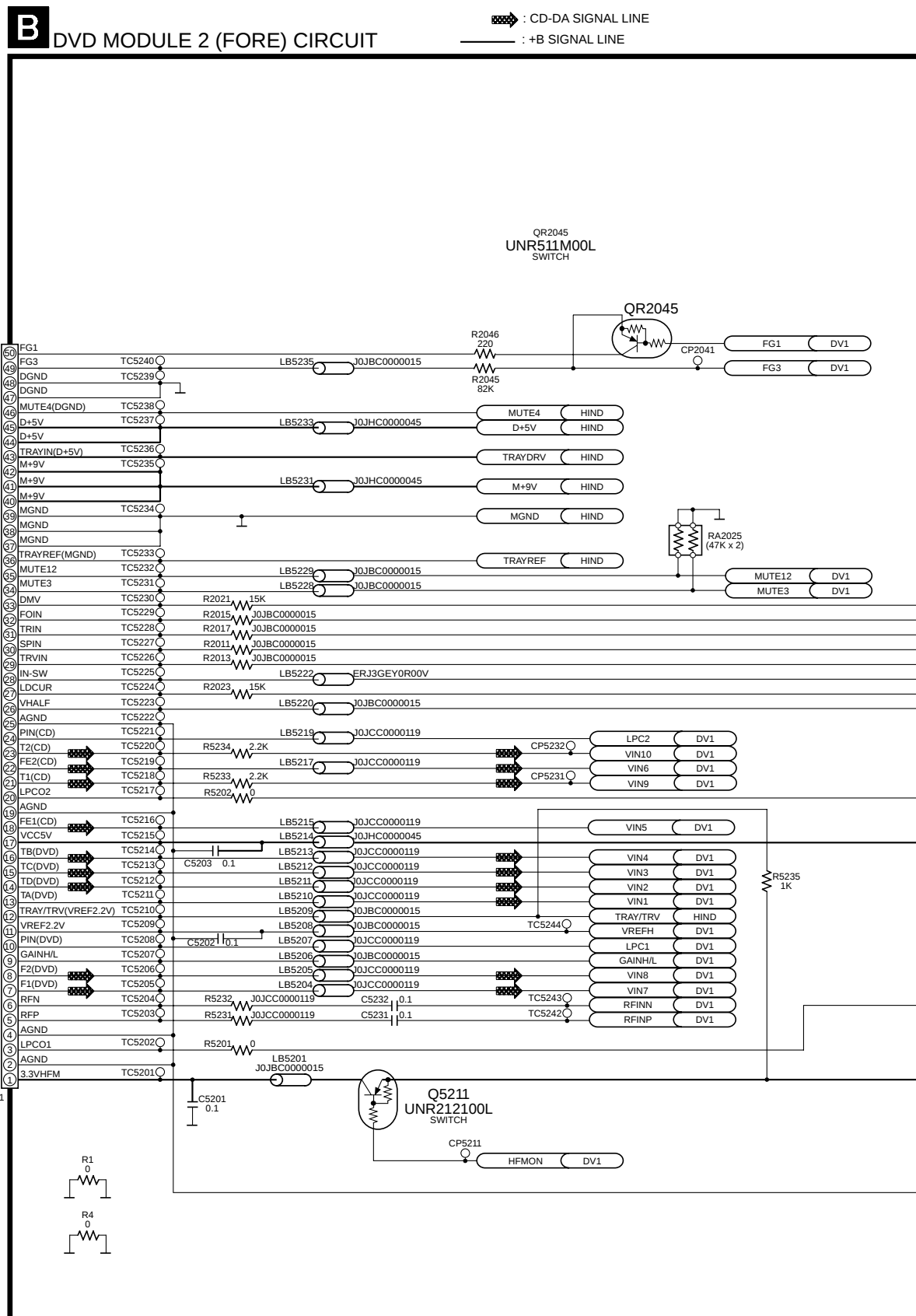
SCHEMATIC DIAGRAM - 3
