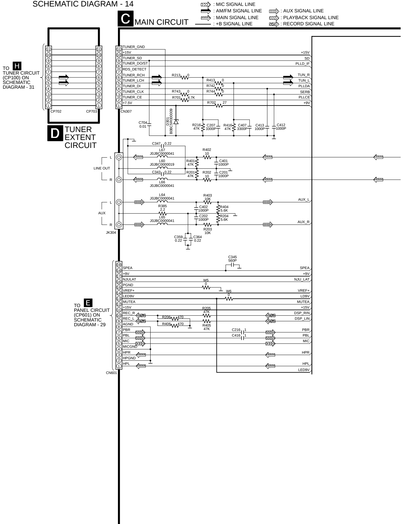
SCHEMATIC DIAGRAM - 14
