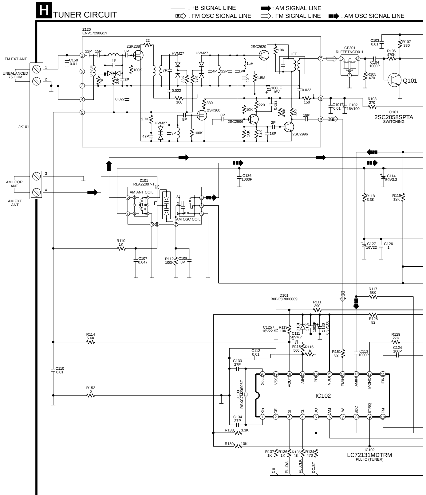
SCHEMATIC DIAGRAM - 30
