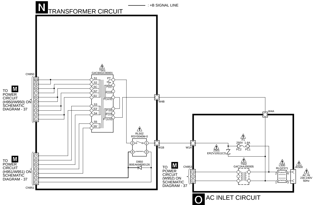
SCHEMATIC DIAGRAM - 38
