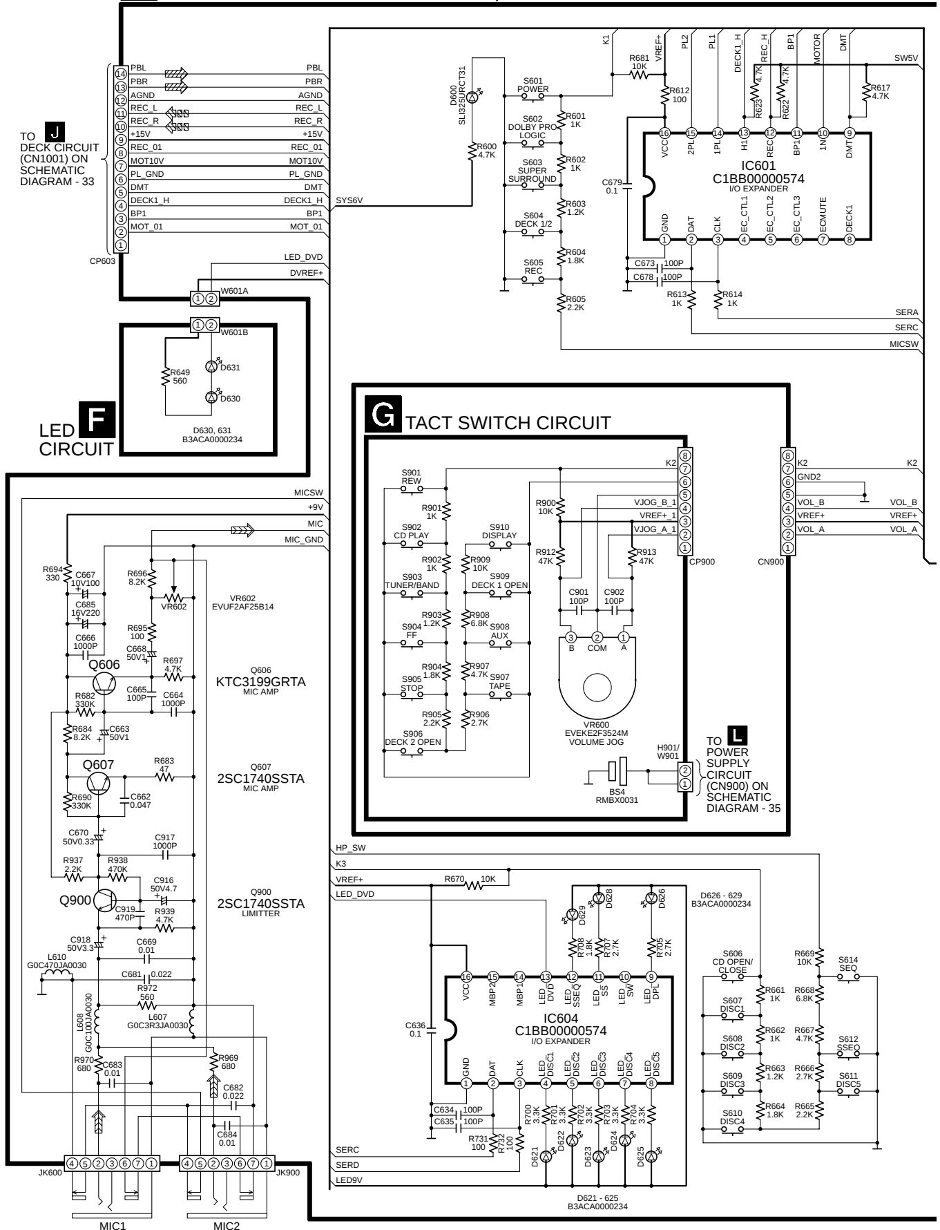
SCHEMATIC DIAGRAM - 26
