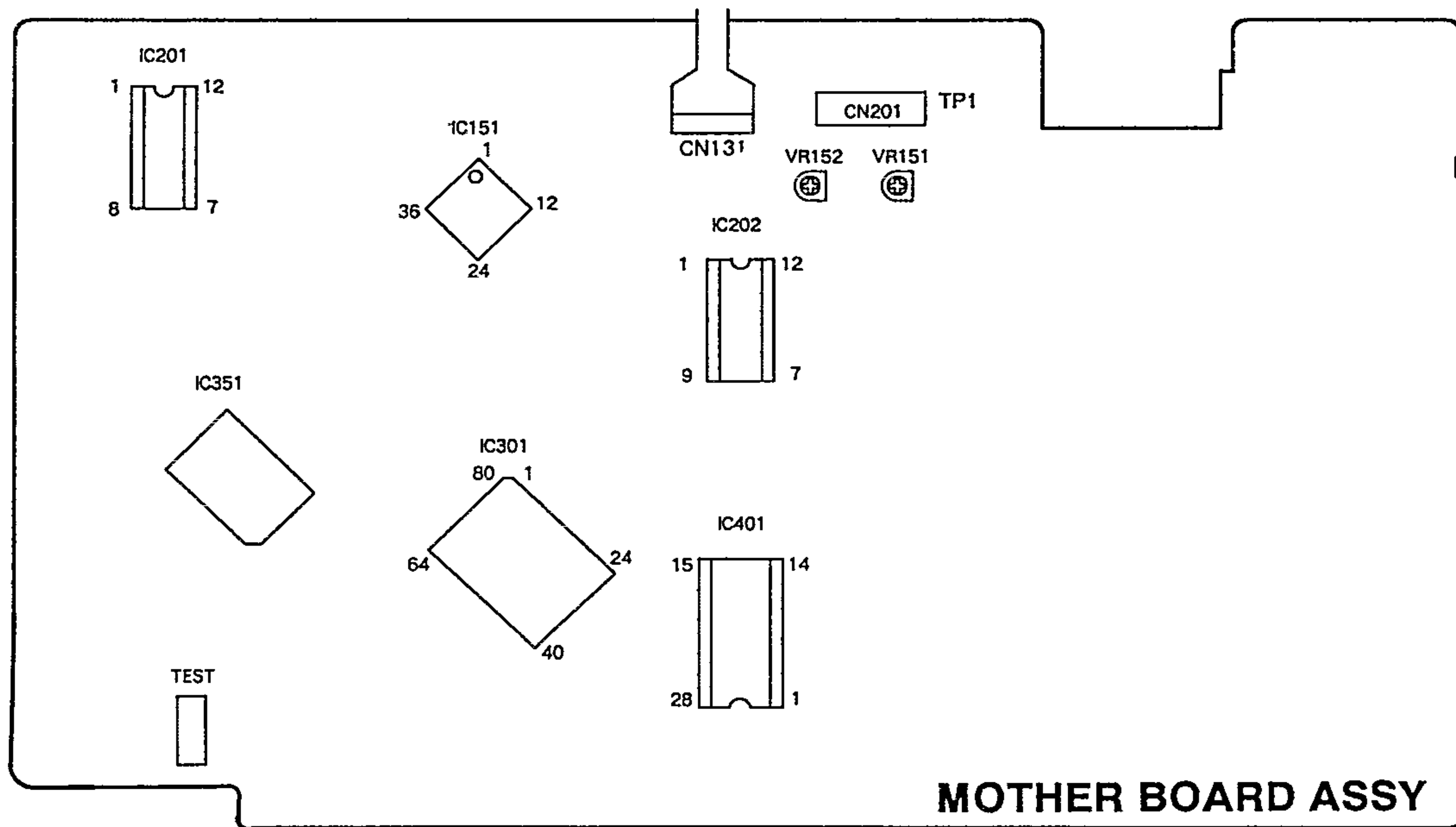
Fig. 1 Adjustment Locations
